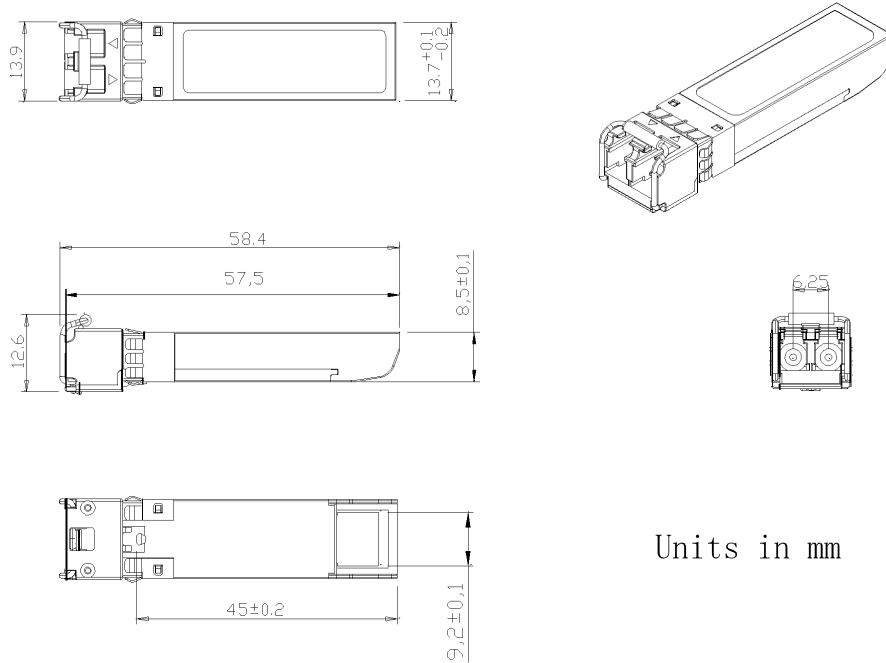
SFP-1G-13-10K-D
